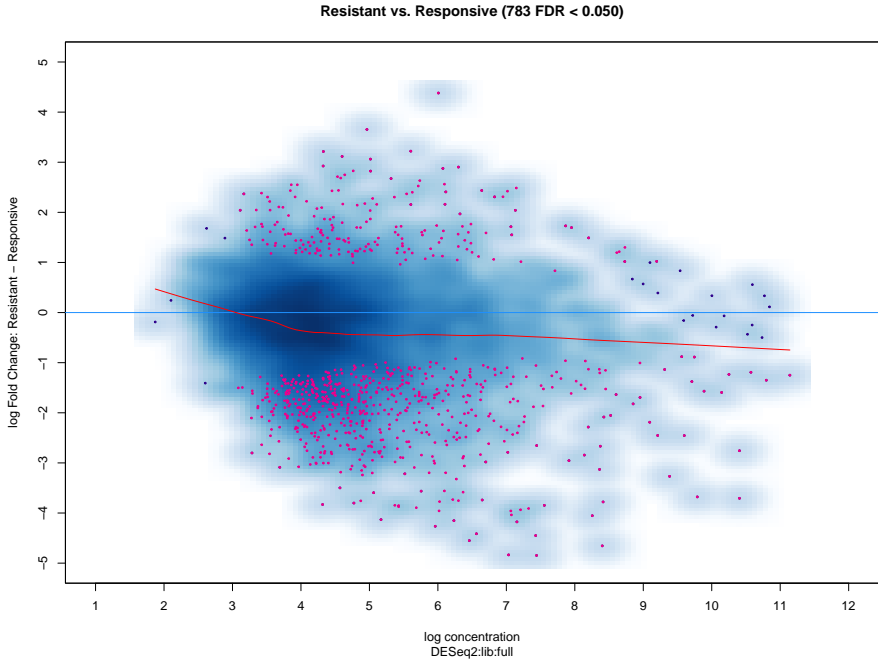
Figure 18: MA plot showing results of analysis using Library-size based normalization.
