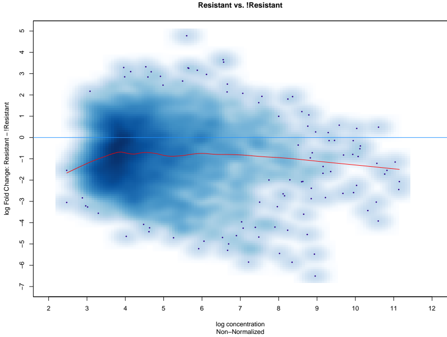
Figure 17: MA plot showing non-normalized data Generated by plotting the result of: dba.plotMA(tamoxifen,contrast=list(Resistant=tamoxifen$marks$Resistant),bNormalized=FALSE,sub="Non-Normalized")
