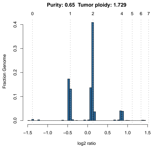
Figure 3: Log-ratio histogram.
