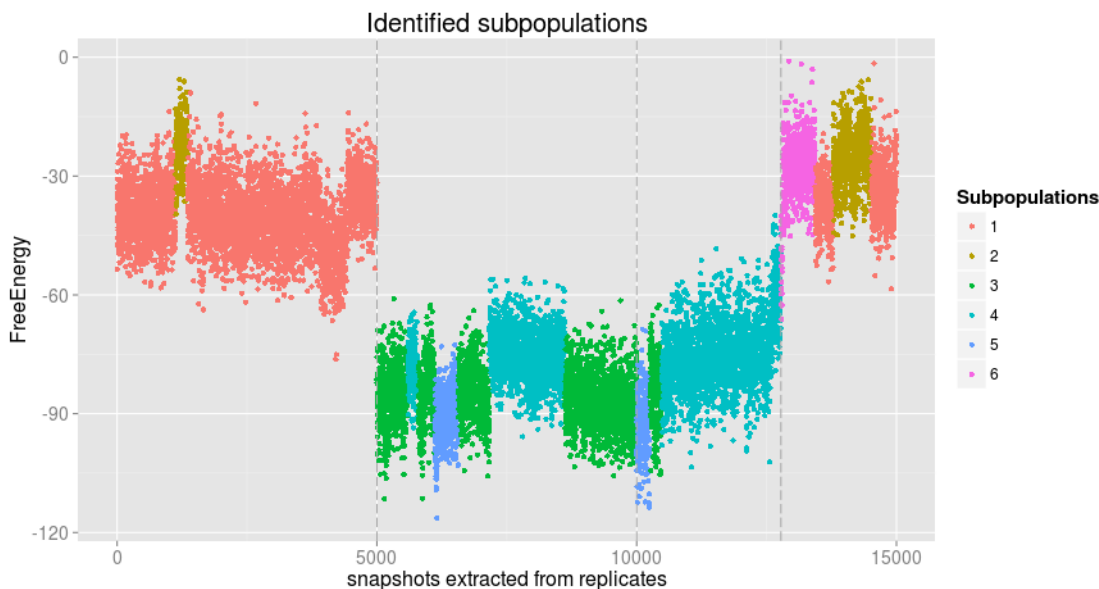
Figure 5: Result of the clusterSegments grouping, with segments coloured according to their respective subpopulations.
