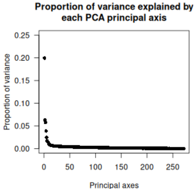
Figure 1: Proportion of variance explained by each principal axis obtained by a Principal Component Analysis (PCA) of the expression matrix.
