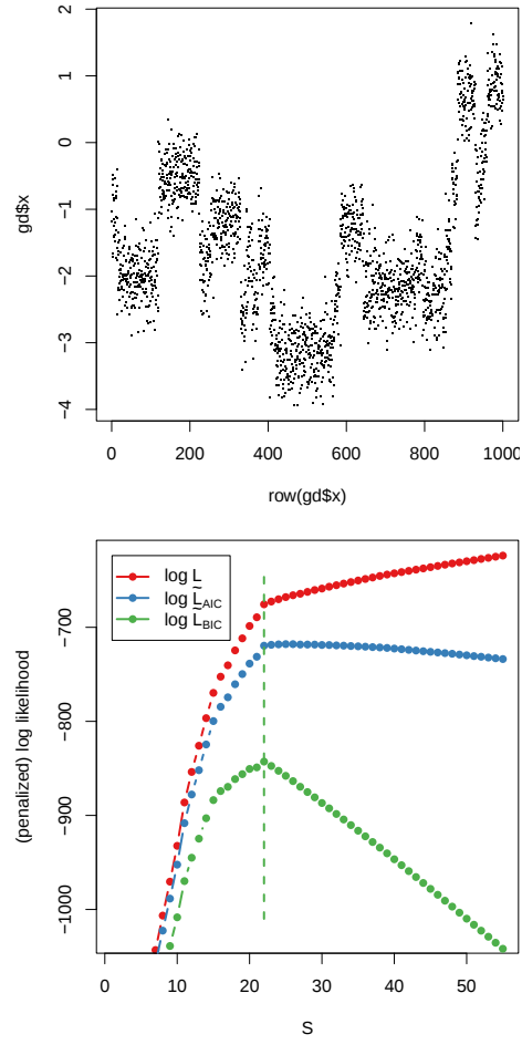
Figure 2: a) simulated data example with nrSeg=22 segments and vertical lines representing the fitted model with S = 22 , selected by maximum \log L_{\text{BIC}} . b) log-likelihood \log L , penalized likelihoods \log \tilde{L}_{\text{AIC}} and \log \tilde{L}_{\text{BIC}} .
