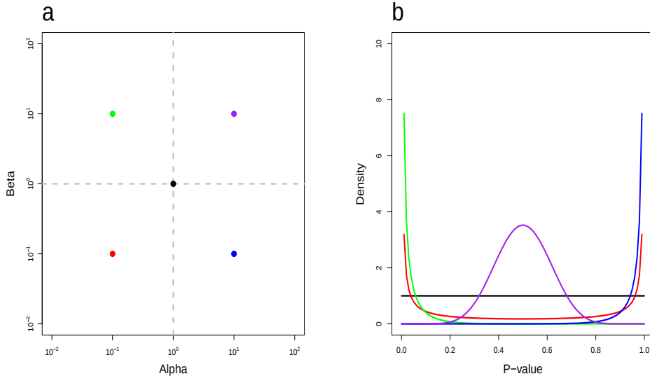
Figure 2: a. The parameter space for the beta distribution, with different parameter combinations highlighted. b. The beta density for the values of (\alpha, \beta) highlighted in a . The densities mimic the behavior of p-values observed in high-dimensional multiple testing experiments.
